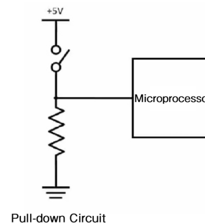
Pull-down Circuit
