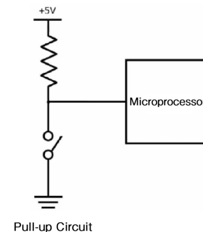
Pull-up Circuit
