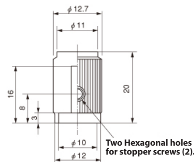
Aluminum Knurring Finish (Silver) Indicator Line: Black Parts Number: 68254908
