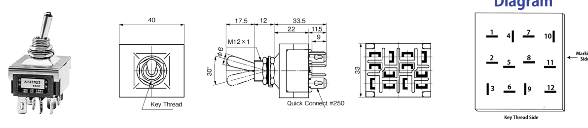
Terminal Diagram
